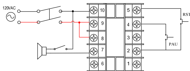
Figure 4. Wiring example of JSL-71.
