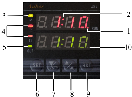
Figure 1. Front Panel of JSL-71.
