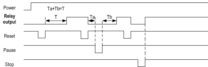
B. single delay (delay on)
