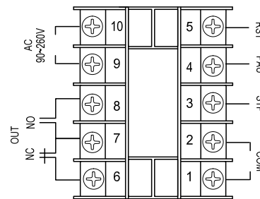
Figure 2. Terminal assignment of JSL-71.
