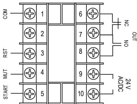
Figure 2. Terminal assignment of JSL-73C-24.
