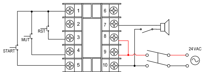
Figure 3. Wiring example of JSL-73C-24.
