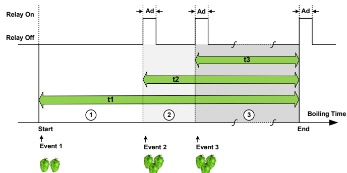
Figure 3. A schematic diagram of how the event timers and the relay work on JSL-73C-24 timer.
