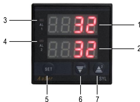
Figure 2. Front panel
