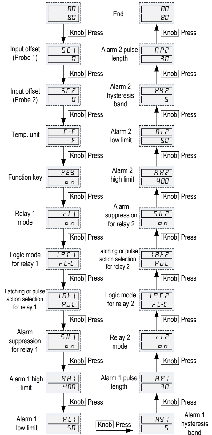
Figure 4. Flow chart of accessing system parameters.
