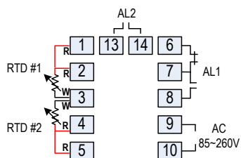
Figure 1. Wiring terminals of SYL-2802.
