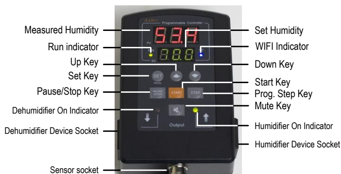
Figure 1. Front Panel.
