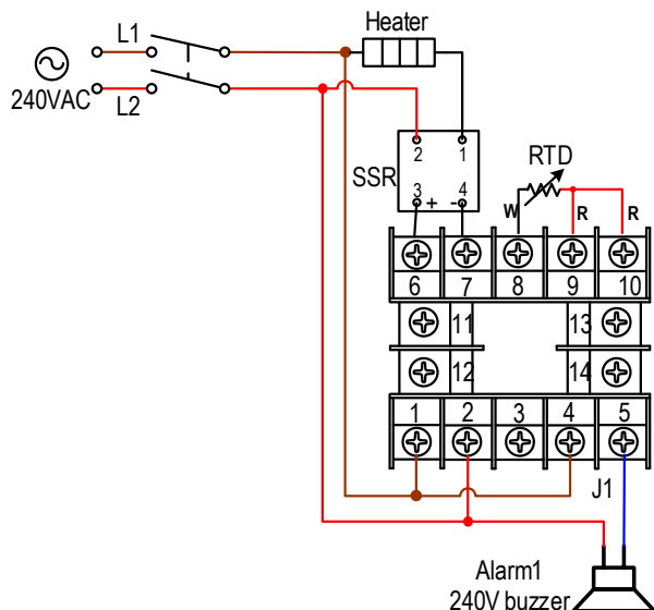
Figure 11. Typical wiring set up for beer brewing and bird incubator. For smoker control, the RTD sensor should be replaced by K type thermocouple
