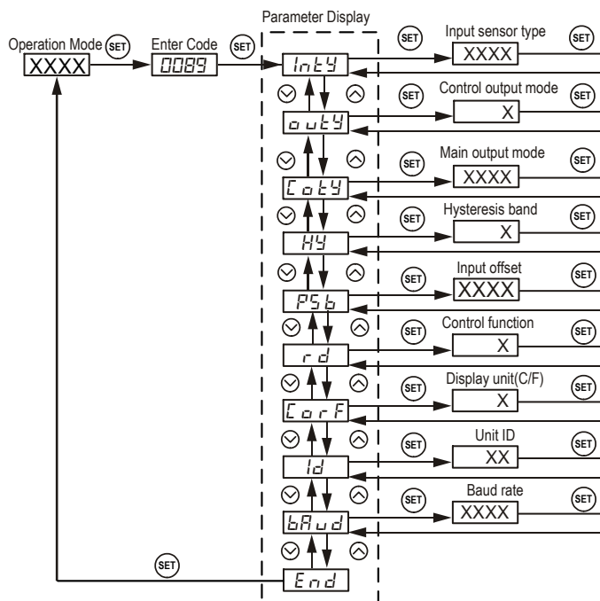
Figure 3. System parameters setup flow chart.
