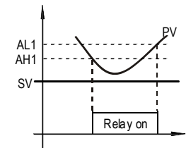
Figure 6. Absolute low alarm
