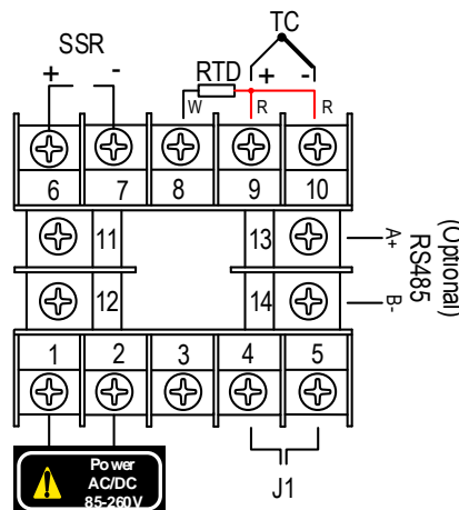
Figure 2. Terminal assignment of SYL-2381-SSR.
