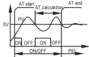
Figure 8. Auto-tuning.
