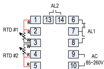
Figure 1. Wiring terminals of SYL-2802B.
