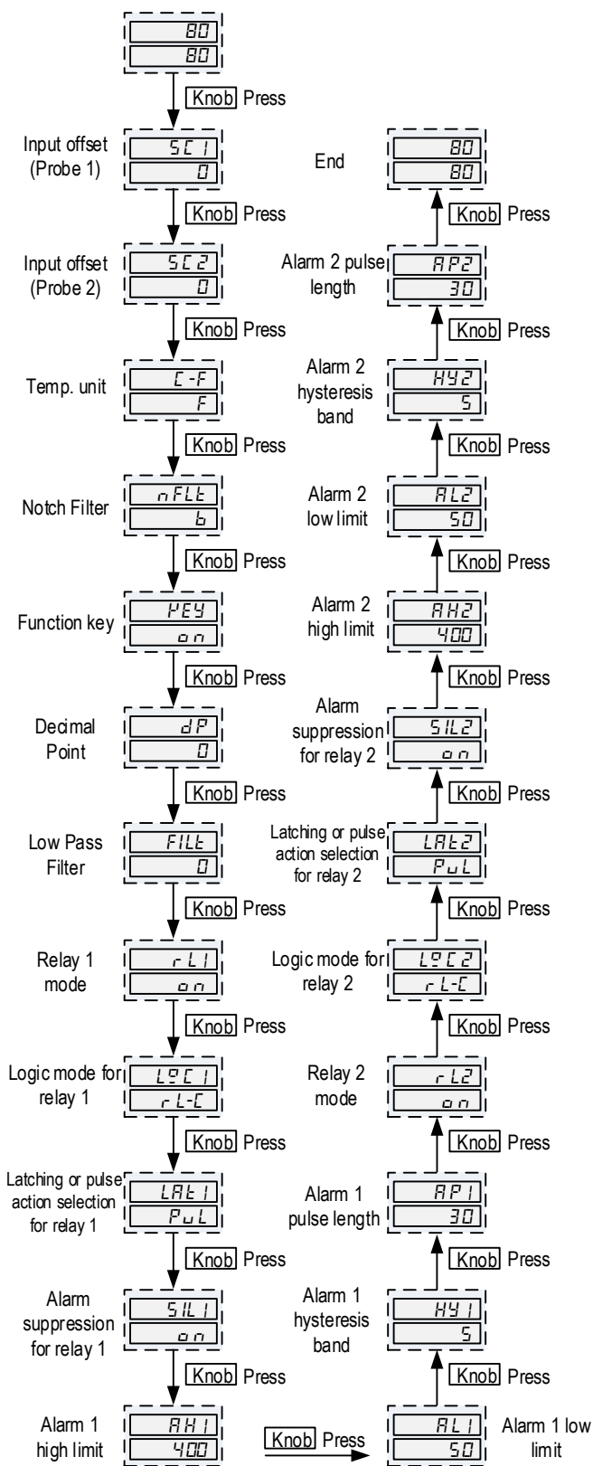
Figure 4. Flow chart of accessing system parameters.
